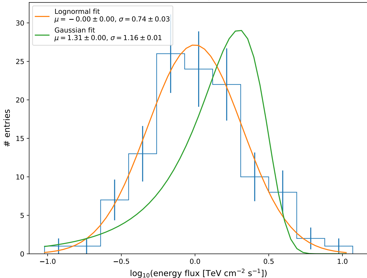
BLLac, cadence - 60 min 2 times per month - CTAO simulation
